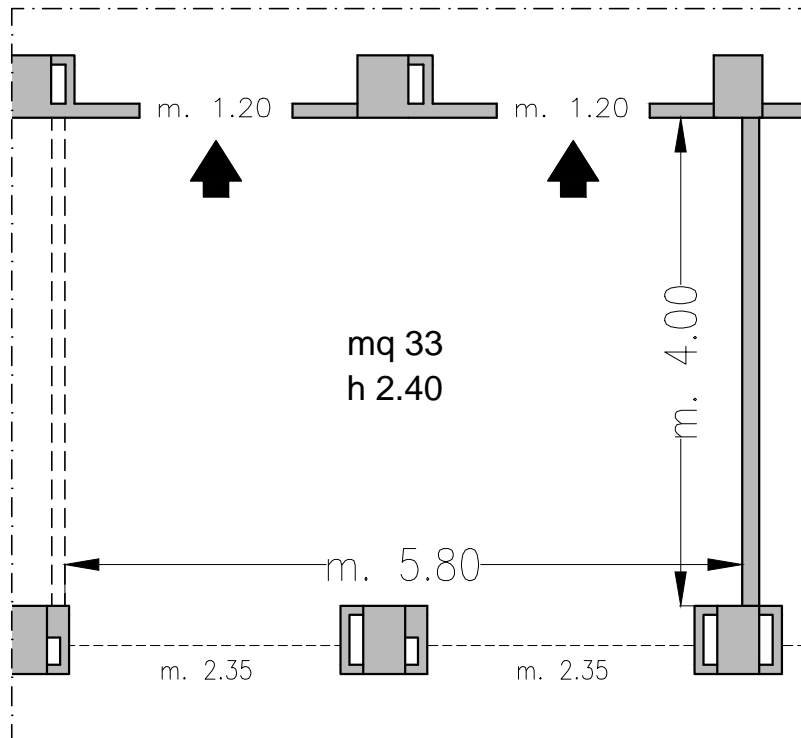
Piano -1 / Basement
